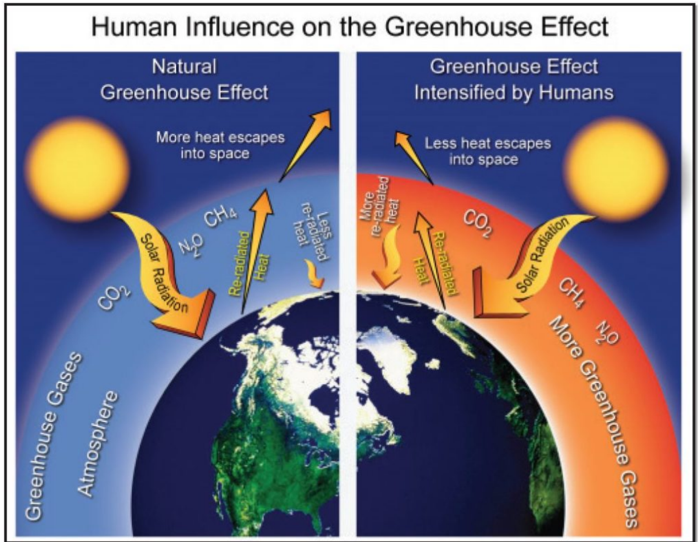
Figure 13.4 | Natural and anthropogenically-forced greenhouse effect
